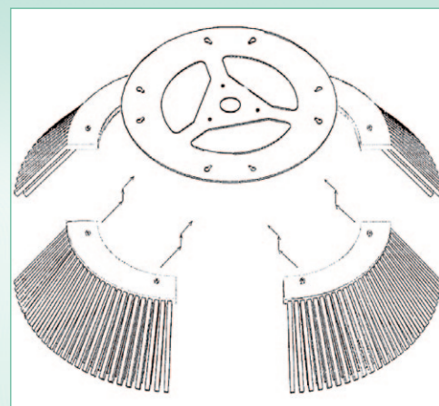
Adjustable brush top, allowing quick assembly for brushes in segments
