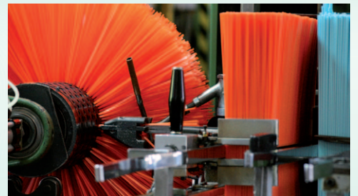
Fixing helicoidal and straight ends
